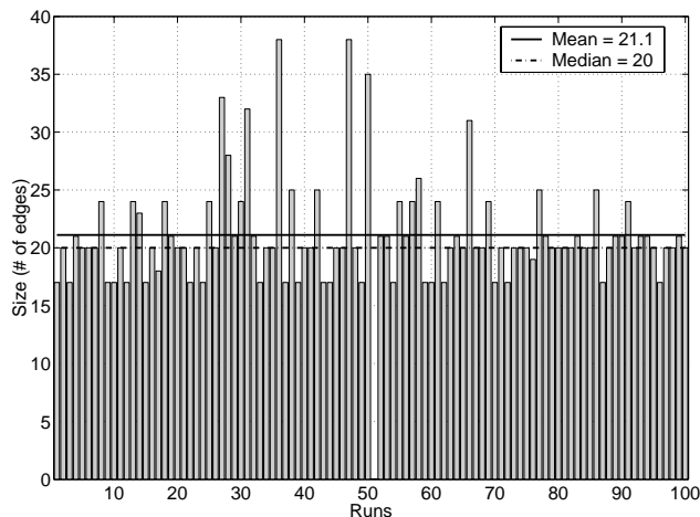
Figure 8: SPEA2, size of the smallest correct solution.
